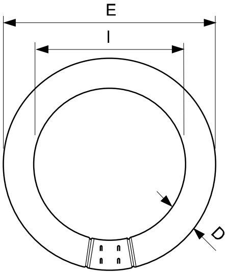
G10q, C-T9
